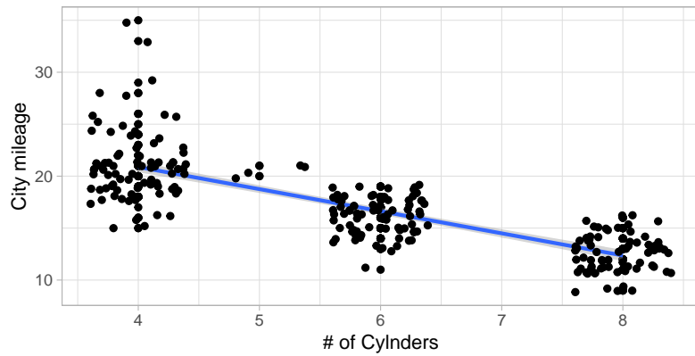
City Mileage versus Cylinders Scatter and jitter plot with regression line
